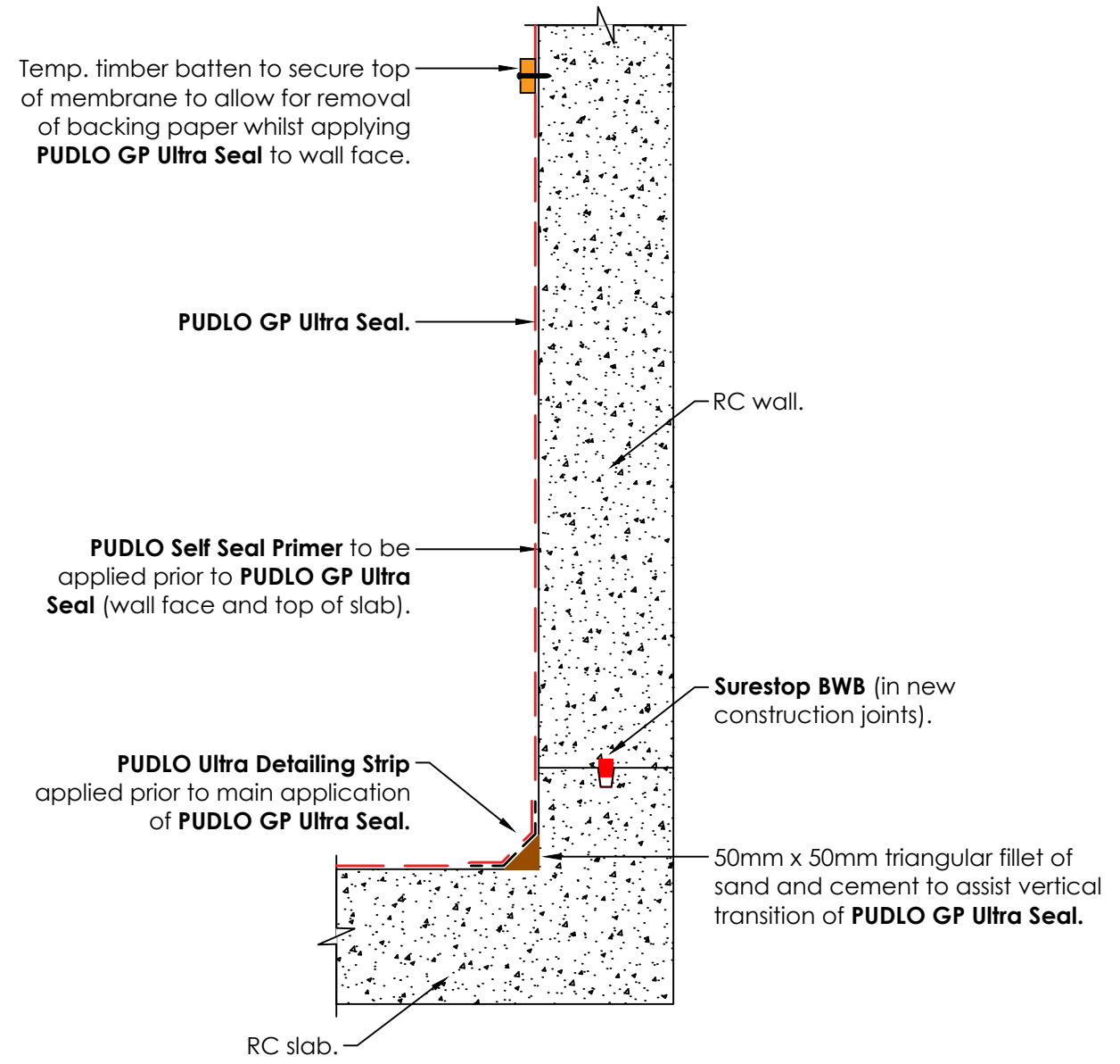
1 Section Elevation Detail Scale: 1:10
